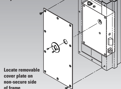
Hinge-side frame mounting, keyed two sides
