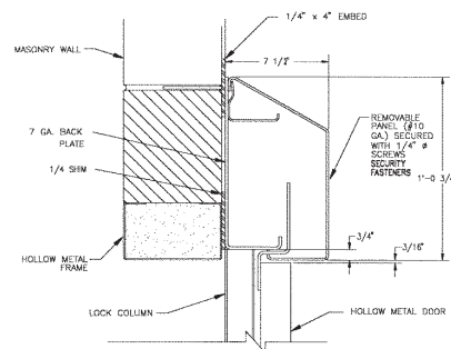
DETAIL A - SLOPED BOX
