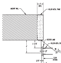
DETAIL C - RECEIVER
