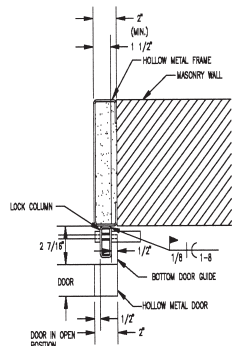
DETAIL B - VERTICAL LOCK JAMB BAR
